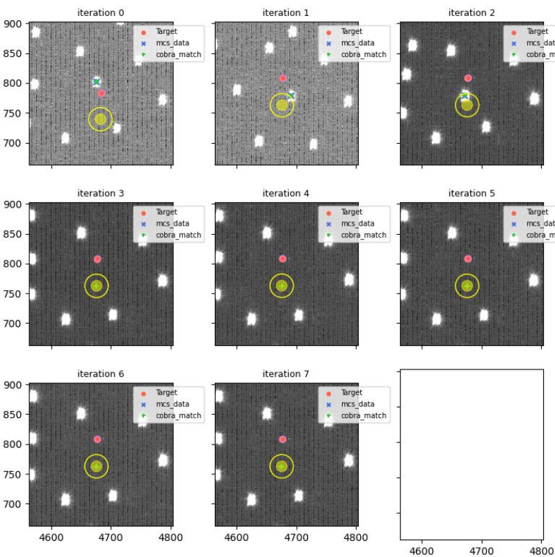
visit=114533 (for 114535), fiberId=2293, Cobrald=1499
