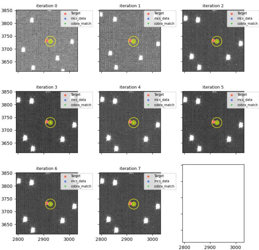
visit=114108 (for 114119), fiberId=1695, Cobrald=552
