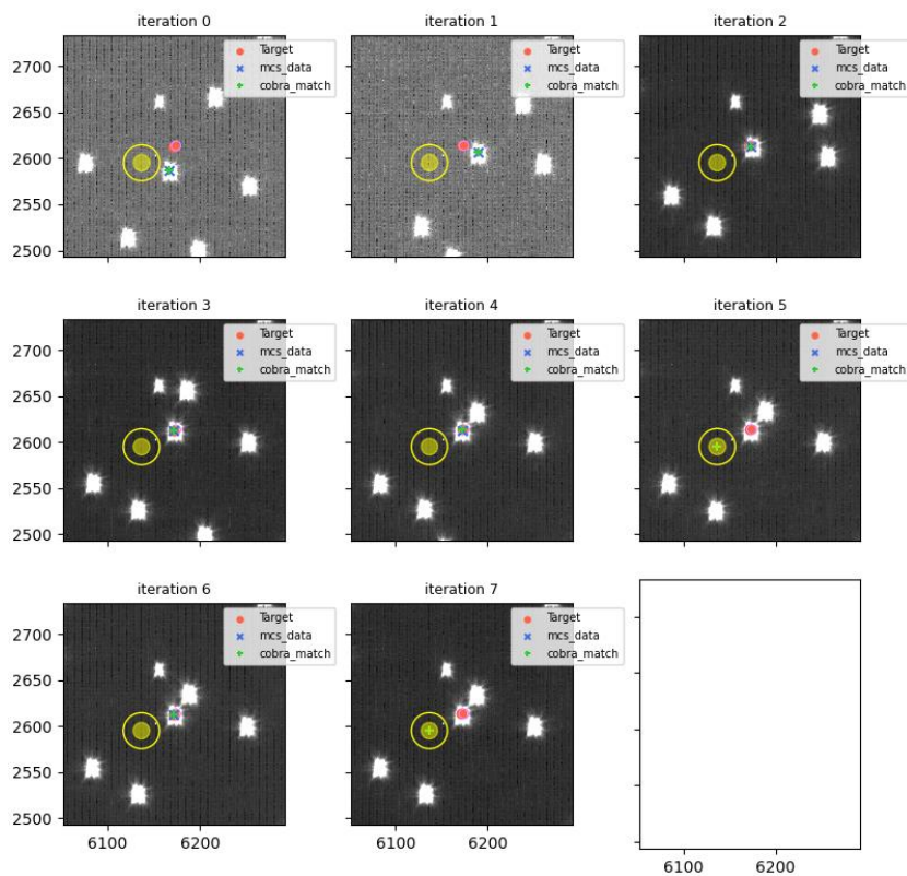
visit=115080 (for 115081), fiberId=1458, Cobrald=2112
