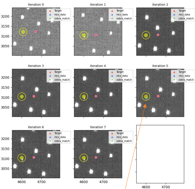
visit=114139 (for 114141), fiberId=1963, Cobrald=9
