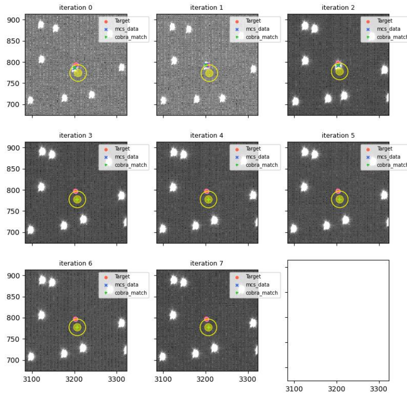
visit=114131 (for 114133), fiberId=344, Cobrald=1588
