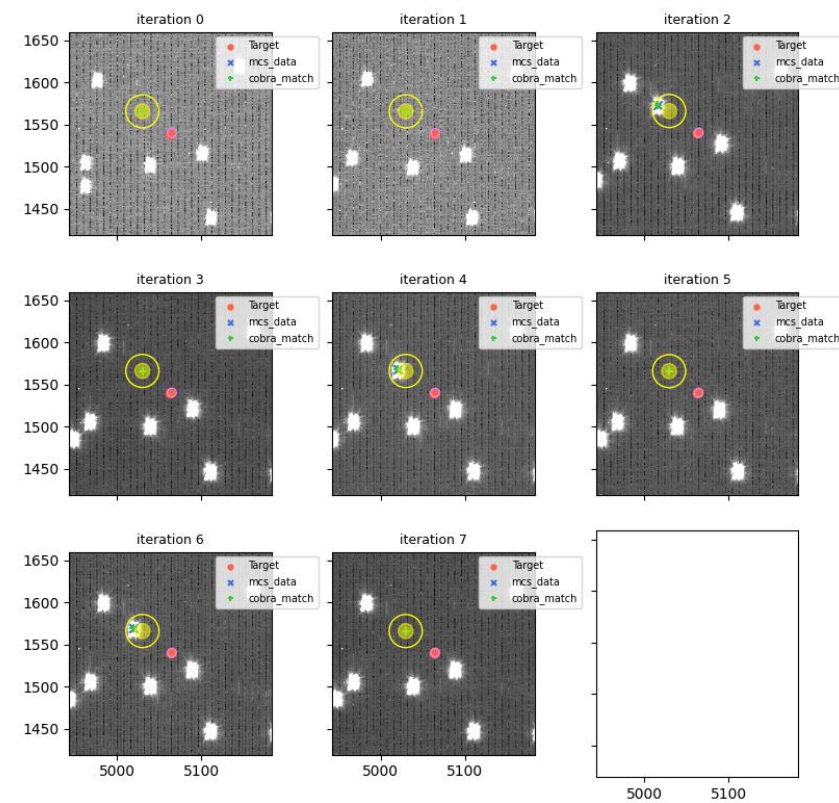
visit=114863 (for 114865), fiberId=1838, Cobrald=1916
