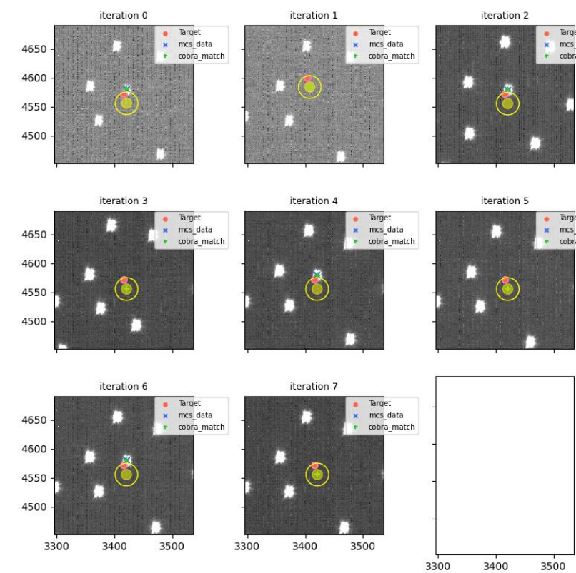
visit=114739 (for 114741), fiberId=390, Cobrald=663
