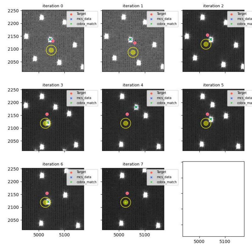
visit=115065 (for 115066), fiberId=1385, Cobrald=1675
