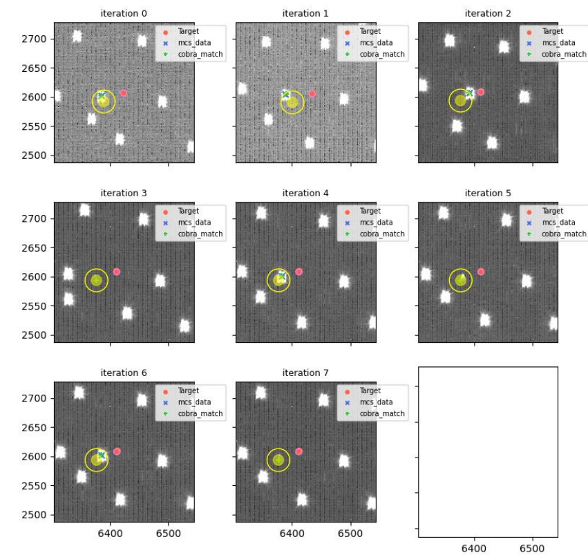
visit=114731 (for 114733), fiberId=1106, Cobrald=2209
