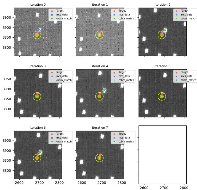
visit=114887 (for 114889), fiberId=1825, Cobrald=1133
