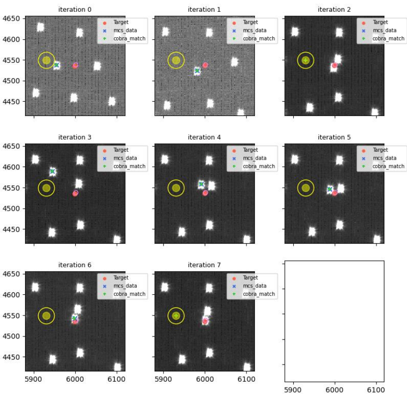
visit=115080 (for 115081), fiberId=407, Cobrald=680
