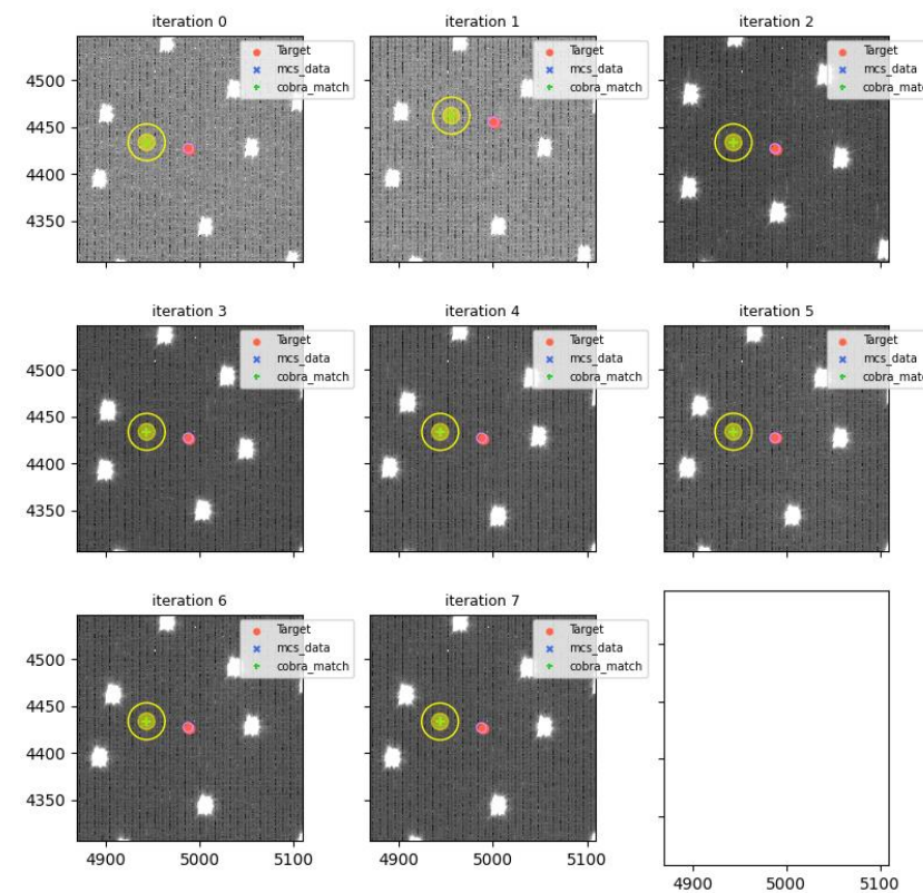
visit=114143 (for 114145), fiberId=1788, Cobrald=328
