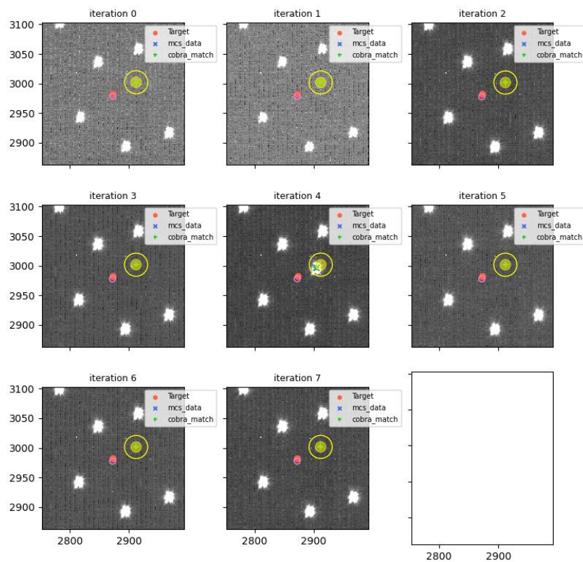
visit=114839 (for 114841), fiberId=1841, Cobrald=1919
