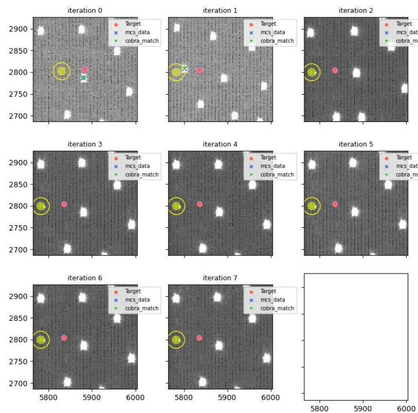
visit=114139 (for 114141), fiberId=645, Cobrald=2019
