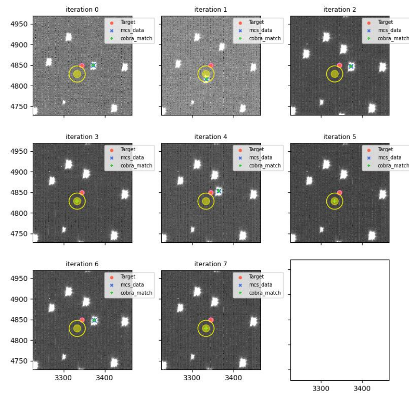
visit=114887 (for 114889), fiberId=2229, Cobrald=687
