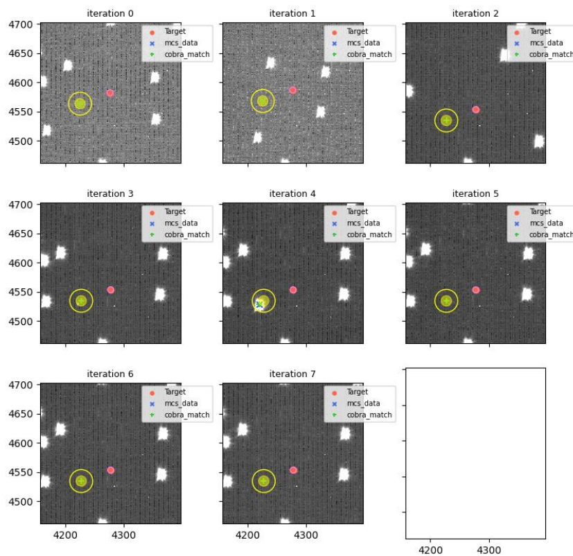
visit=114875 (for 114877), fiberId=2345, Cobrald=494
