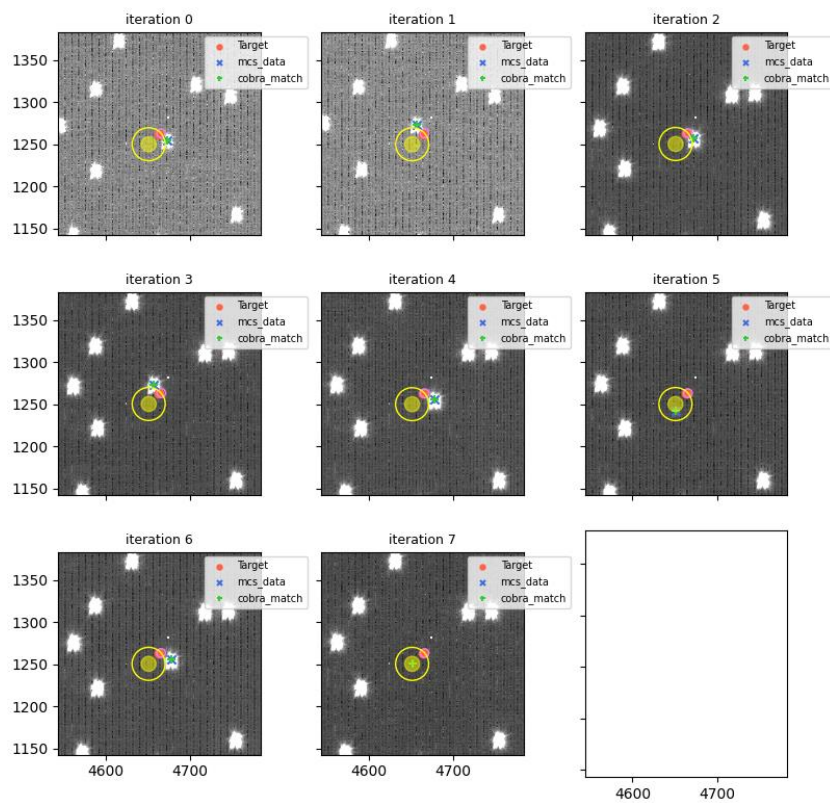
visit=114859 (for 114861), fiberId=903, Cobrald=1748
