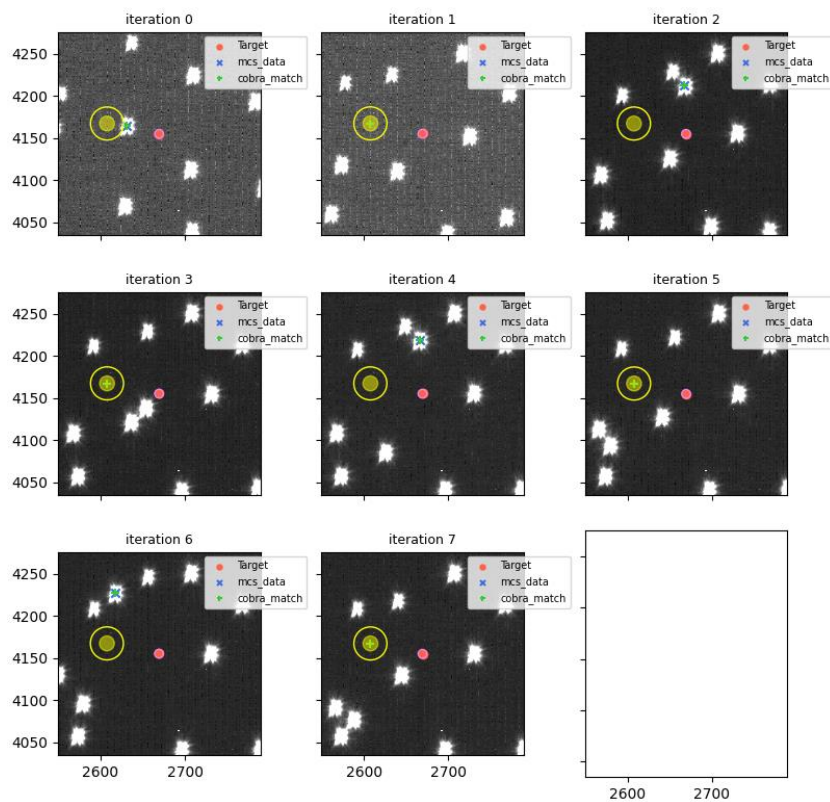
visit=115058 (for 115059), fiberId=2232, Cobrald=690
