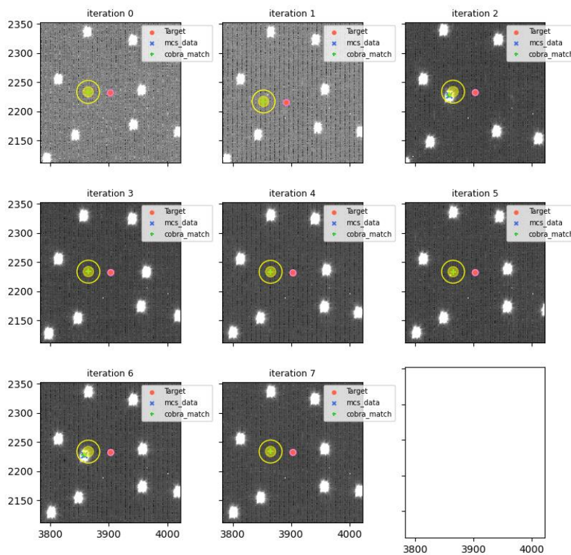
visit=114537 (for 114539), fiberId=50, Cobrald=987
