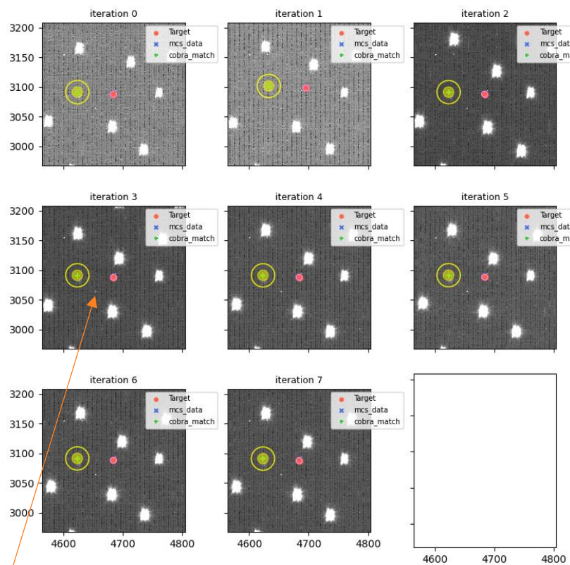
visit=114143 (for 114145), fiberId=1963, Cobrald=9
