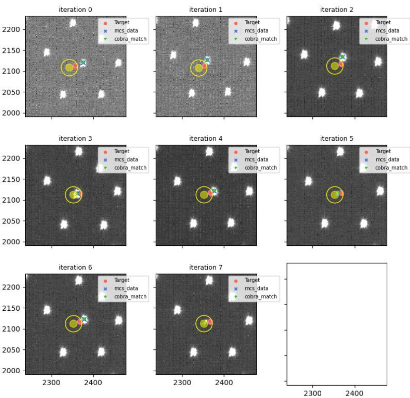
visit=114727 (for 114729), fiberId=2480, Cobrald=1080
