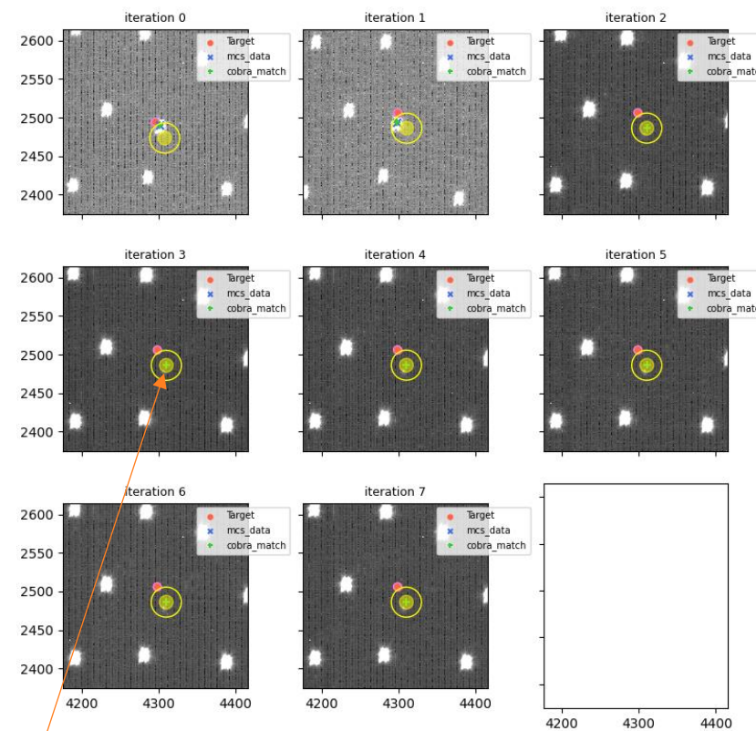
visit=114533 (for 114535), fiberId=1338, Cobrald=861
