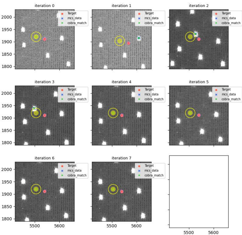
visit=114143 (for 114145), fiberId=1838, Cobrald=1916
