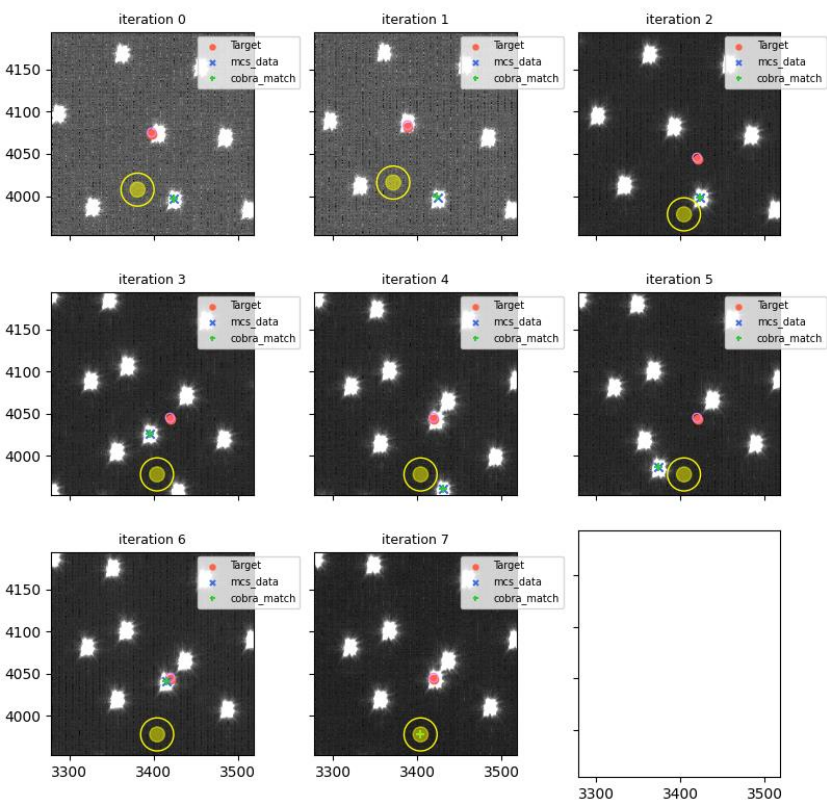
visit=115065 (for 115066), fiberId=1420, Cobrald=538
