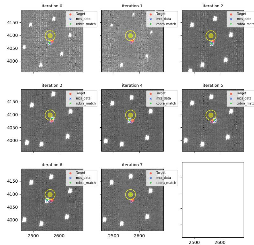
visit=115027 (for 115029), fiberId=919, Cobrald=1764
