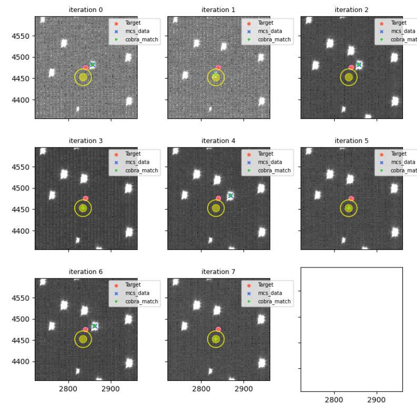
visit=114883 (for 114885), fiberId=2229, Cobrald=687
