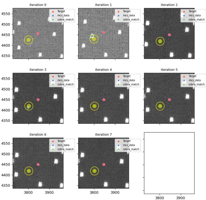
visit=114867 (for 114869), fiberId=2345, Cobrald=494
