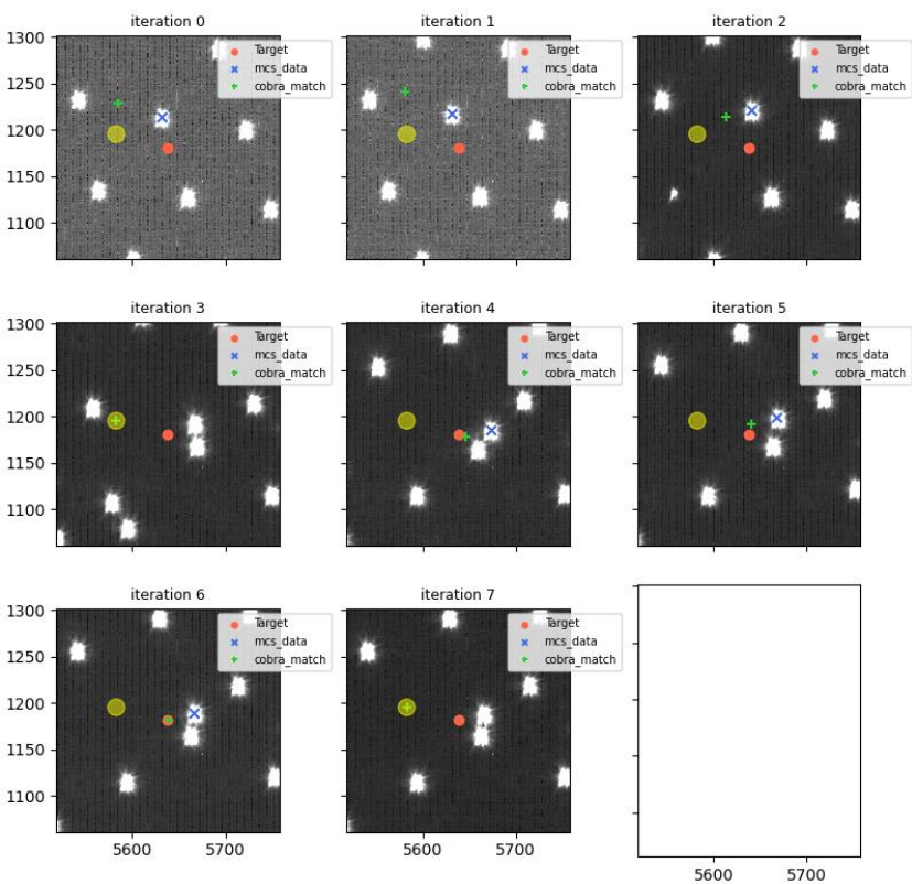
visit=115065 (for 115066), fiberId=263, Cobrald=1816
