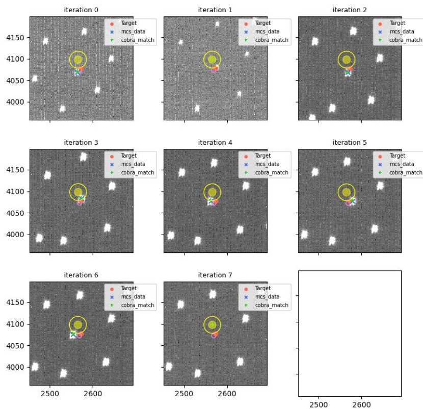
visit=115027 (for 115028), fiberId=919, Cobrald=1764
