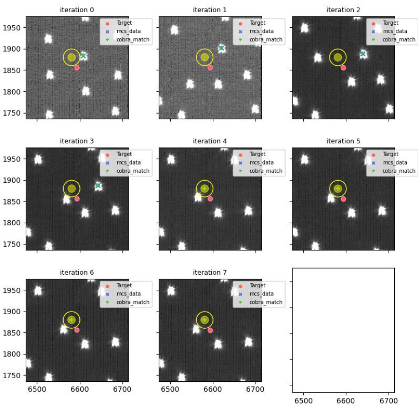
visit=115058 (for 115059), fiberId=371, Cobrald=2384
