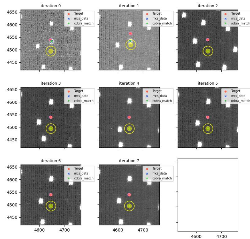
visit=114537 (for 114539), fiberId=1788, Cobrald=328
