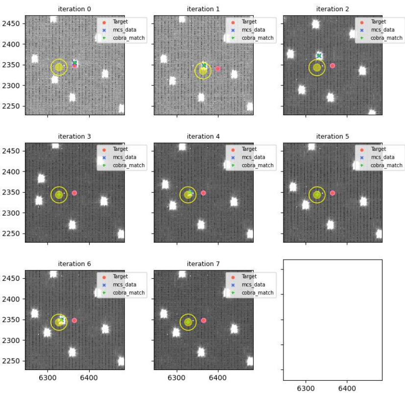
visit=114739 (for 114741), fiberId=1106, Cobrald=2209
