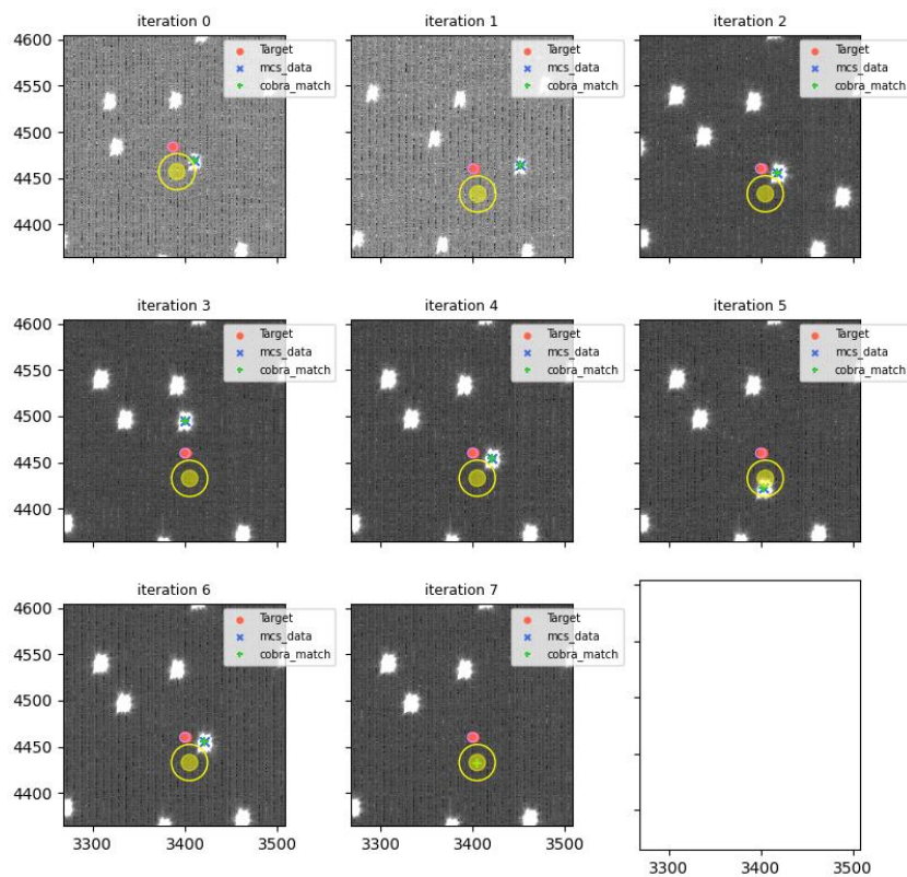
visit=114533 (for 114535), fiberId=1043, Cobrald=608
