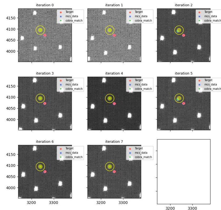
visit=114553 (for 114555), fiberId=2176, Cobrald=837
