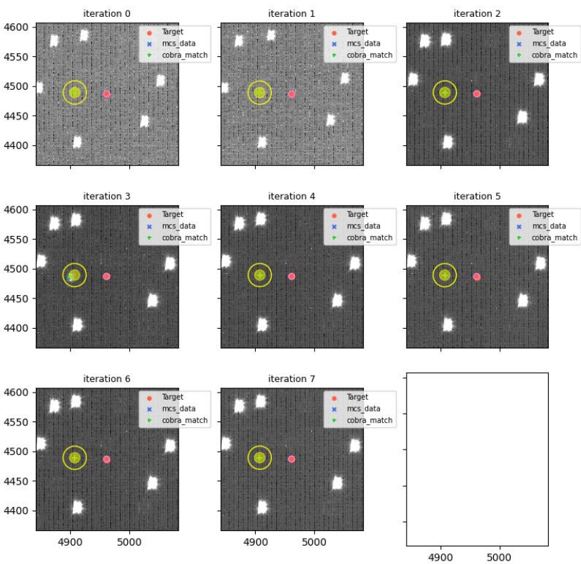
visit=114883 (for 114885), fiberId=2345, Cobrald=494
