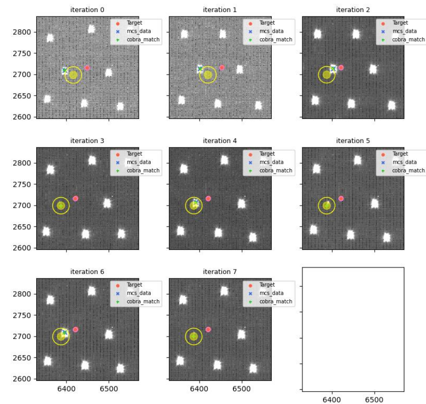
visit=114727 (for 114729), fiberId=1106, Cobrald=2209
