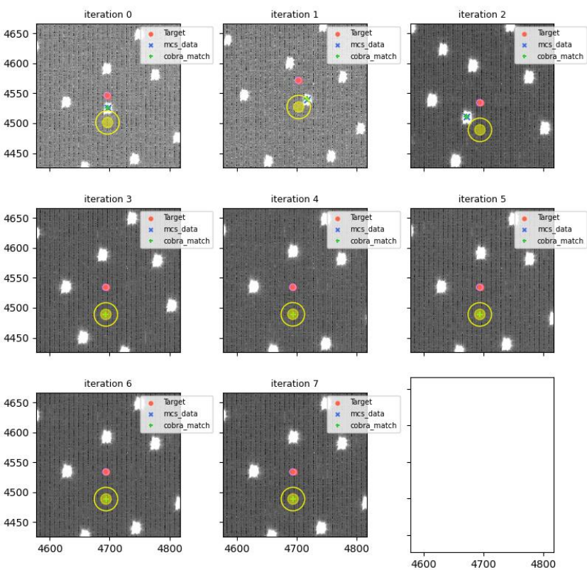
visit=114135 (for 114137), fiberId=1788, Cobrald=328
