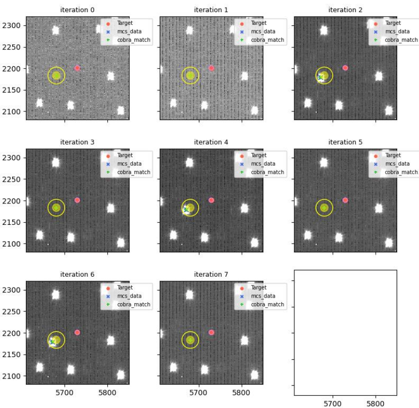
visit=114817 (for 114828), fiberId=1838, Cobrald=1916
