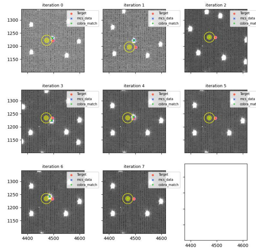
visit=114135 (for 114137), fiberId=1437, Cobrald=1324
