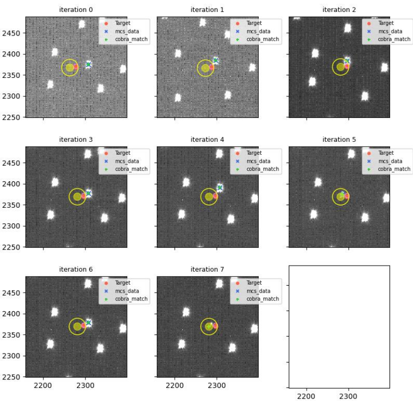
visit=114735 (for 114737), fiberId=2480, Cobrald=1080
