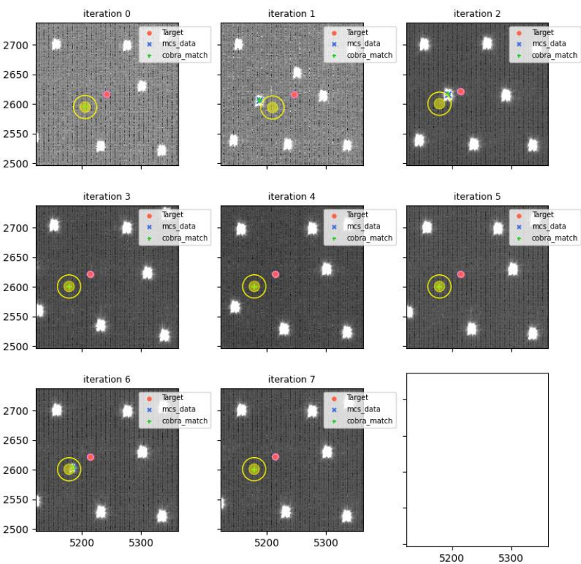
visit=114727 (for 114729), fiberId=80, Cobrald=1786
