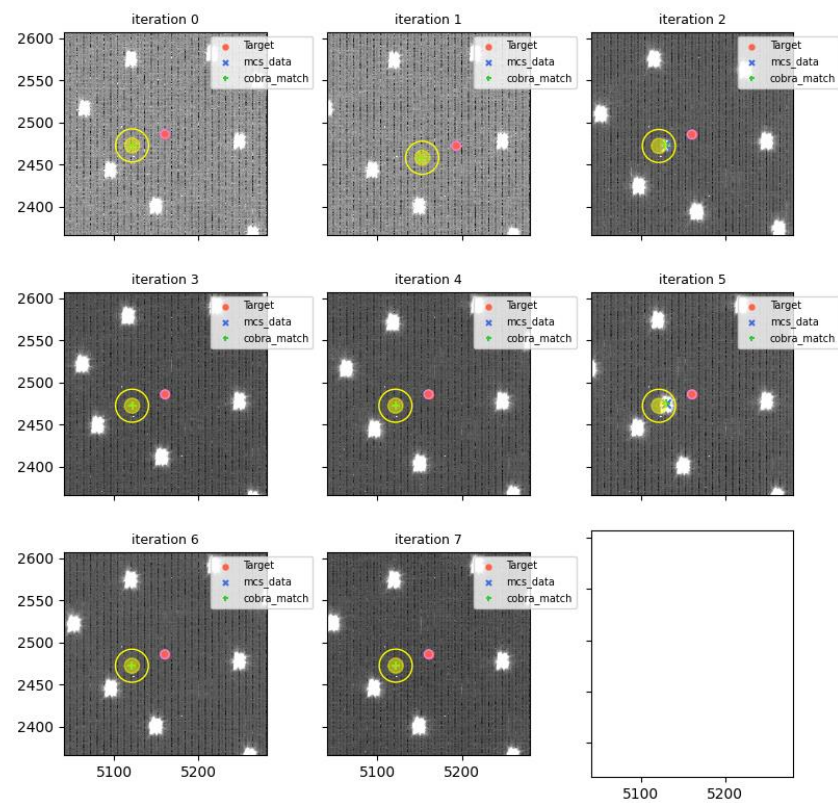
visit=114739 (for 114741), fiberId=80, Cobrald=1786
