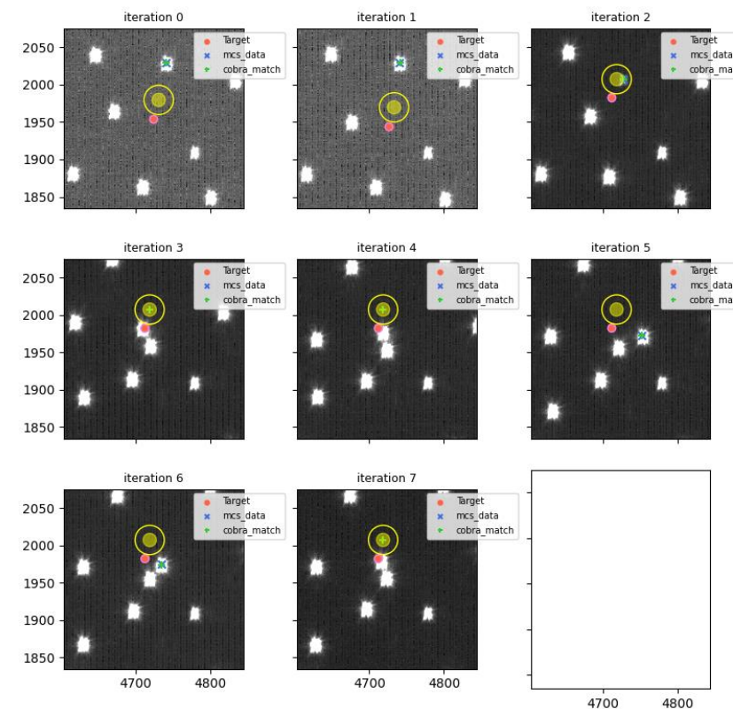
visit=115065 (for 115066), fiberId=2544, Cobrald=1027
