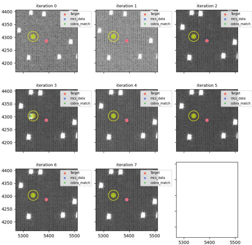
visit=114887 (for 114889), fiberId=2345, Cobrald=494
