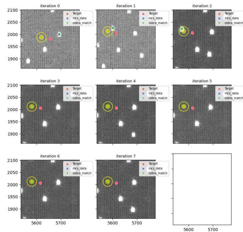
visit=114139 (for 114141), fiberId=1838, Cobrald=1916
