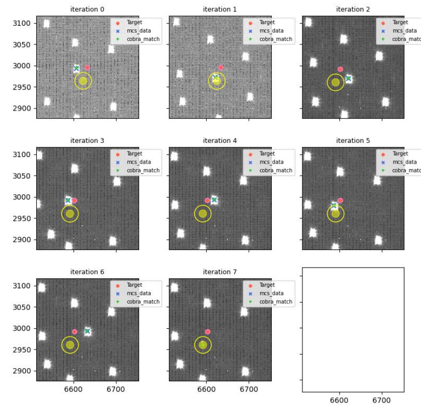
visit=114747 (for 114749), fiberId=1683, Cobrald=2366
