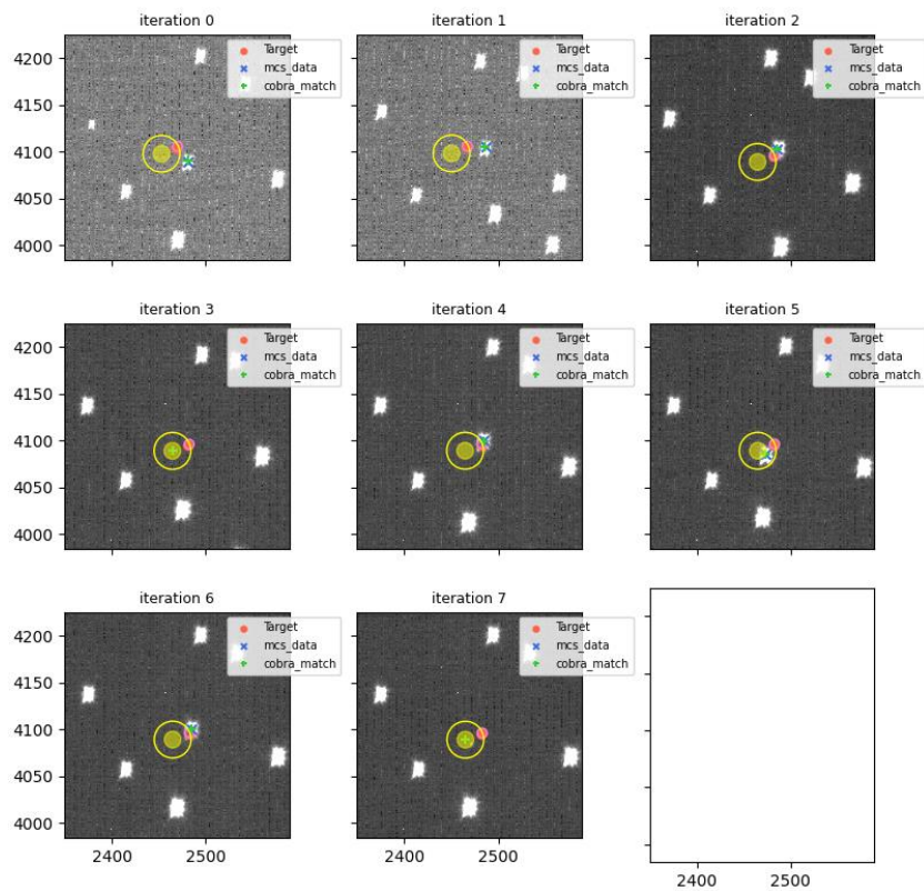
visit=114747 (for 114749), fiberId=1584, Cobrald=750
