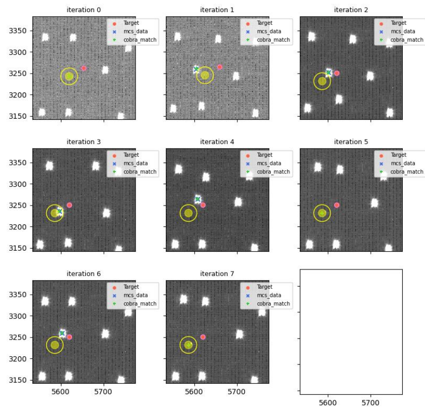
visit=114727 (for 114729), fiberId=640, Cobrald=2014
