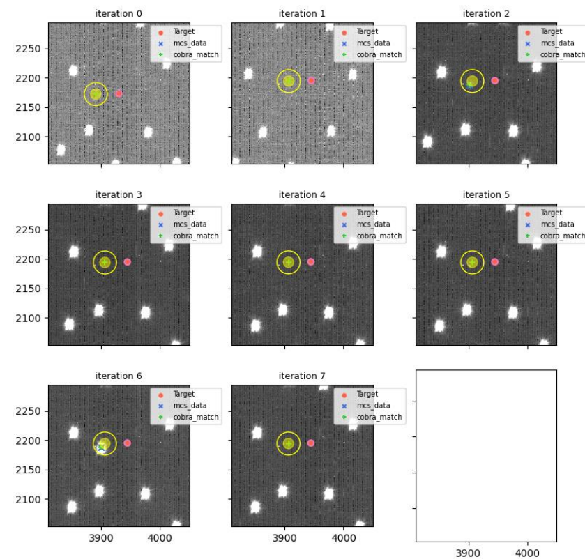
visit=114533 (for 114535), fiberId=50, Cobrald=987
