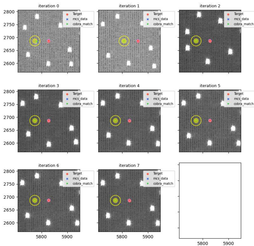
visit=114143 (for 114145), fiberId=645, Cobrald=2019
