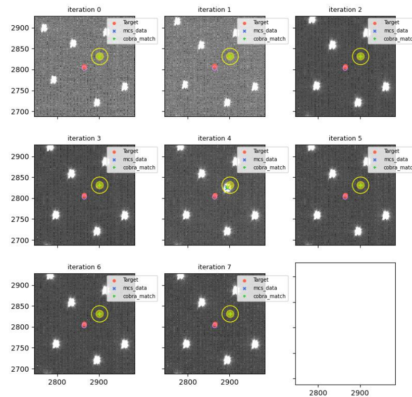
visit=114847 (for 114849), fiberId=1841, Cobrald=1919
