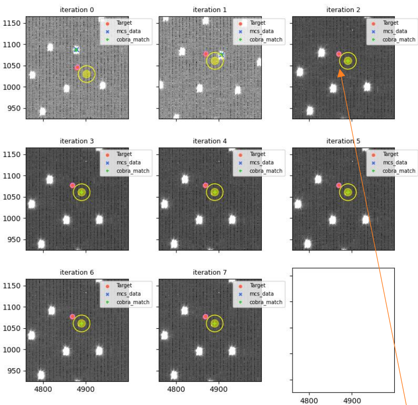
visit=114533 (for 114535), fiberId=782, Cobrald=1377
