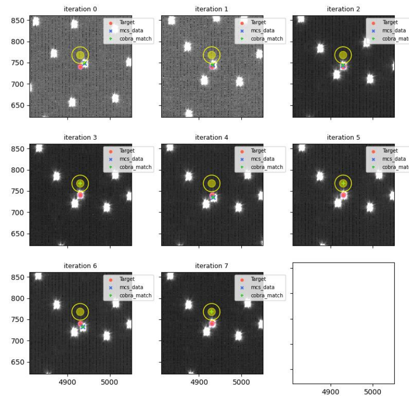
visit=115080 (for 115081), fiberId=1764, Cobrald=2159
