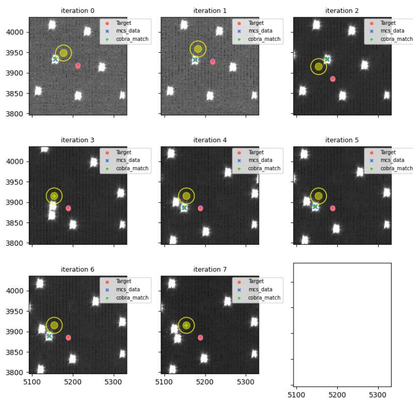
visit=115065 (for 115066), fiberId=2139, Cobrald=30
