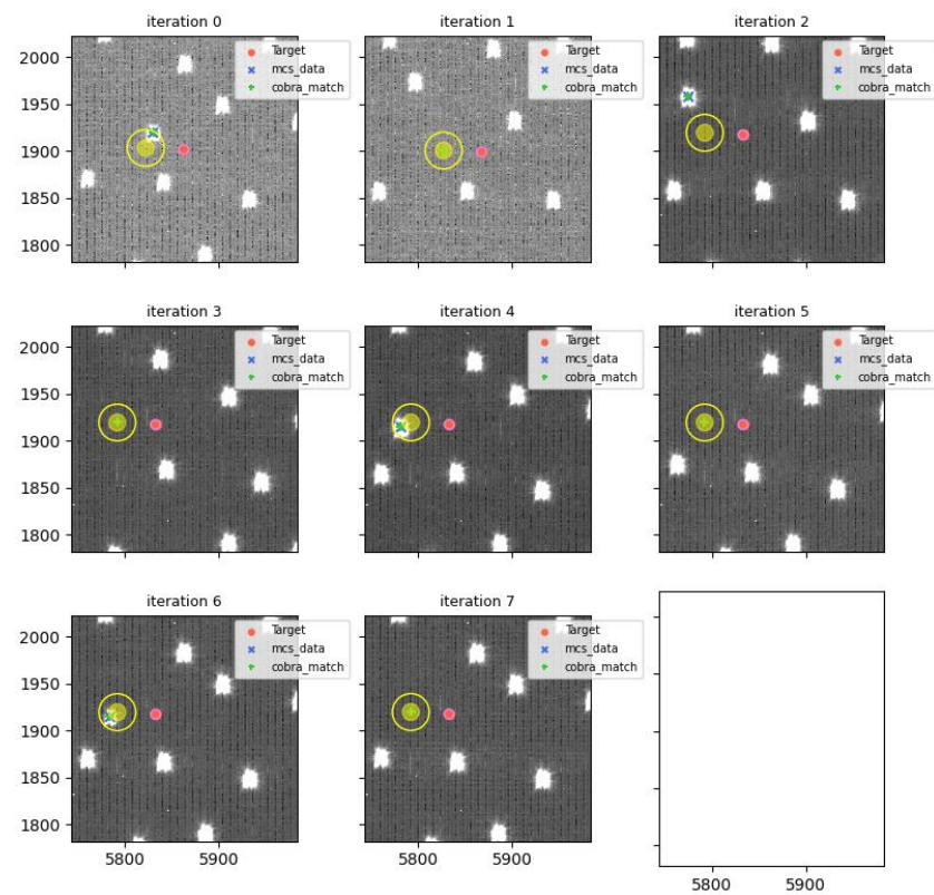
visit=114727 (for 114729), fiberId=2494, Cobrald=1864
