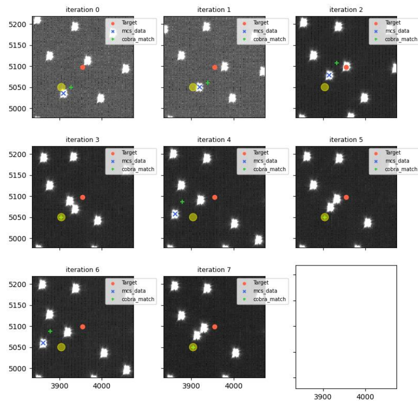
visit=115065 (for 115066), fiberId=407, Cobrald=680
