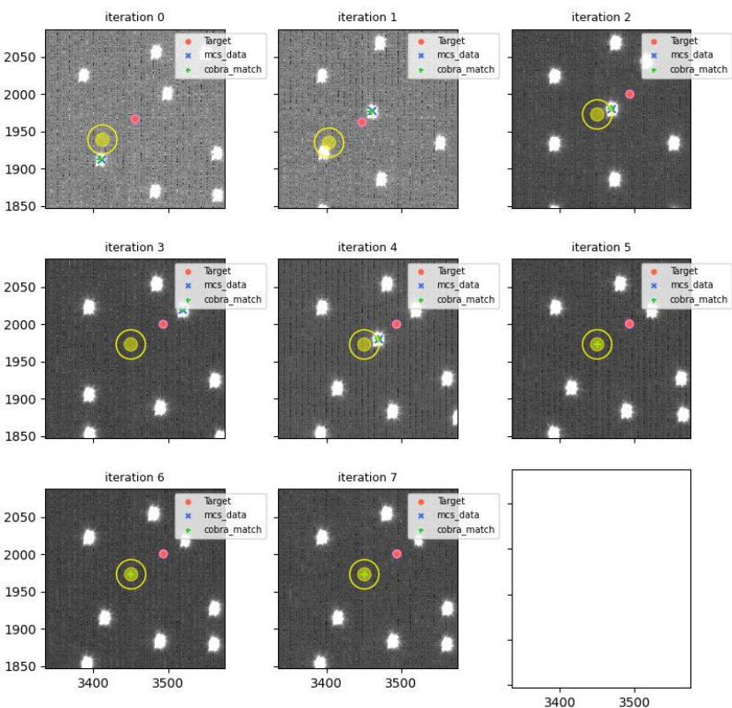
visit=114545 (for 114547), fiberId=617, Cobrald=1222
