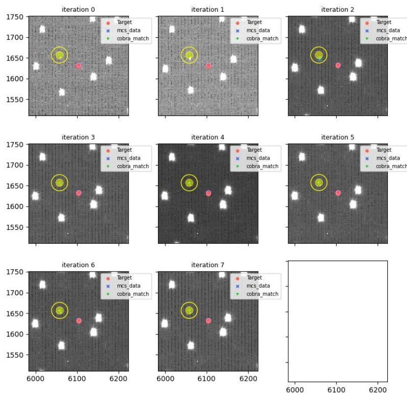
visit=114553 (for 114555), fiberId=448, Cobrald=2259
