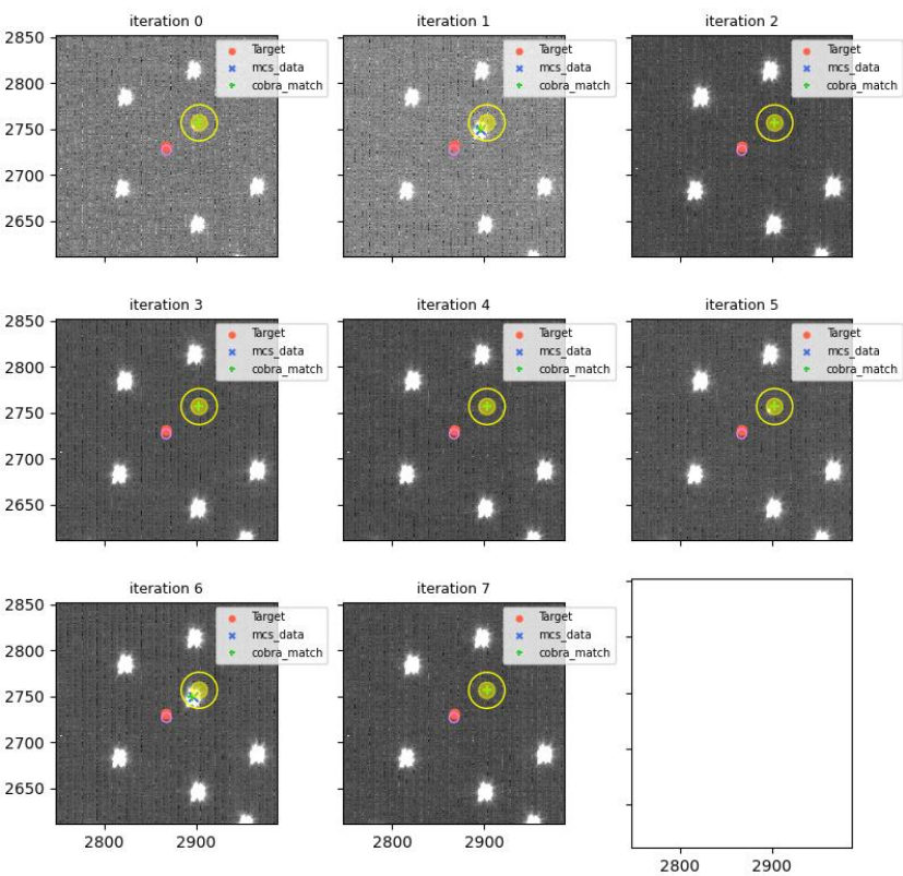
visit=114851 (for 114853), fiberId=1841, Cobrald=1919
