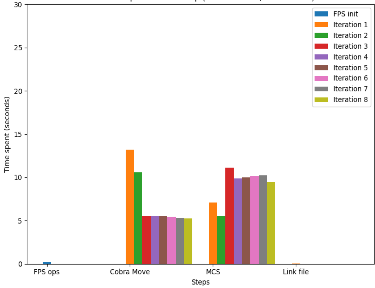
FPS Time spent in each step (visit=110479, t=131.244s)
