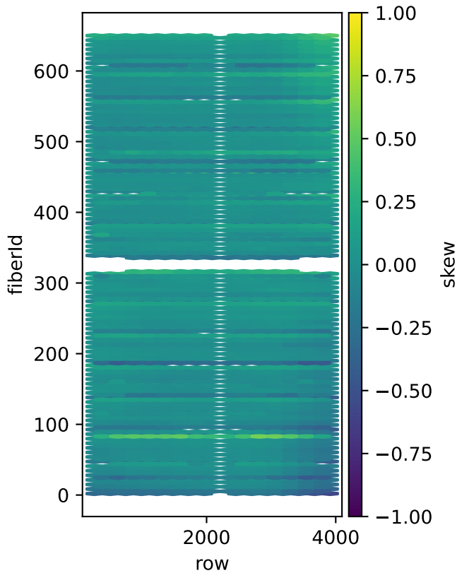
Third moment of the profile, normalised by the second moment
