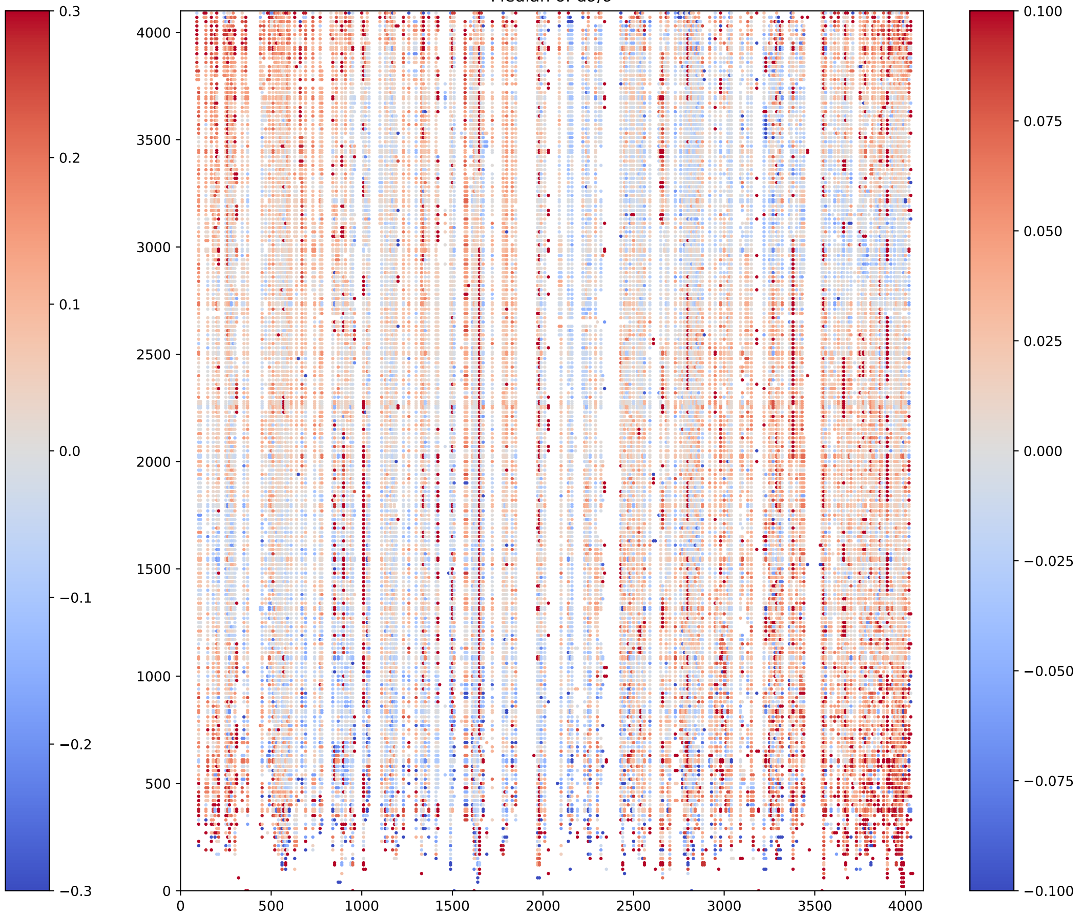
Median of d\sigma/\sigma
