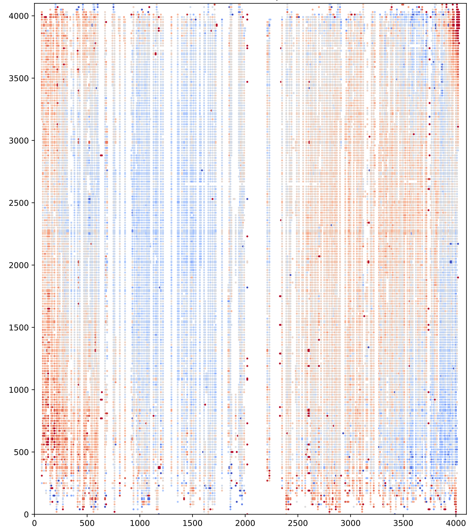
Median of dx (pix)
