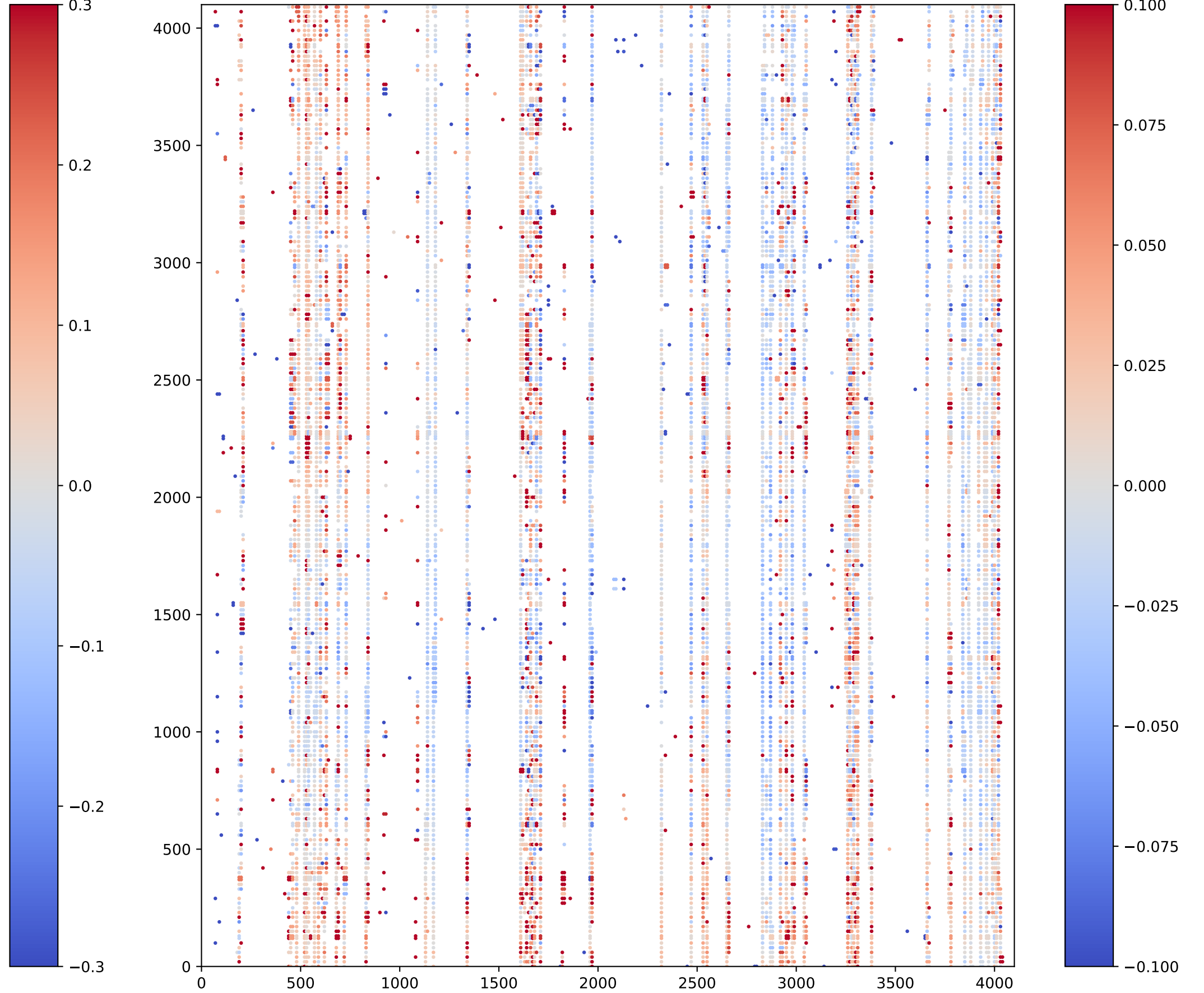
Median of d\sigma/\sigma
