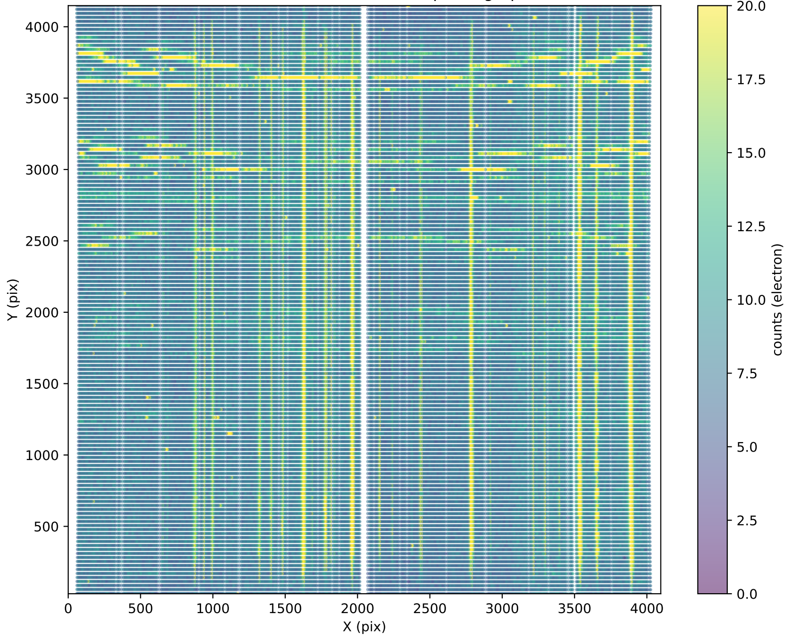
stddev counts in 7x7 cell (visit=98042,spectrograph=1,arm=r)
