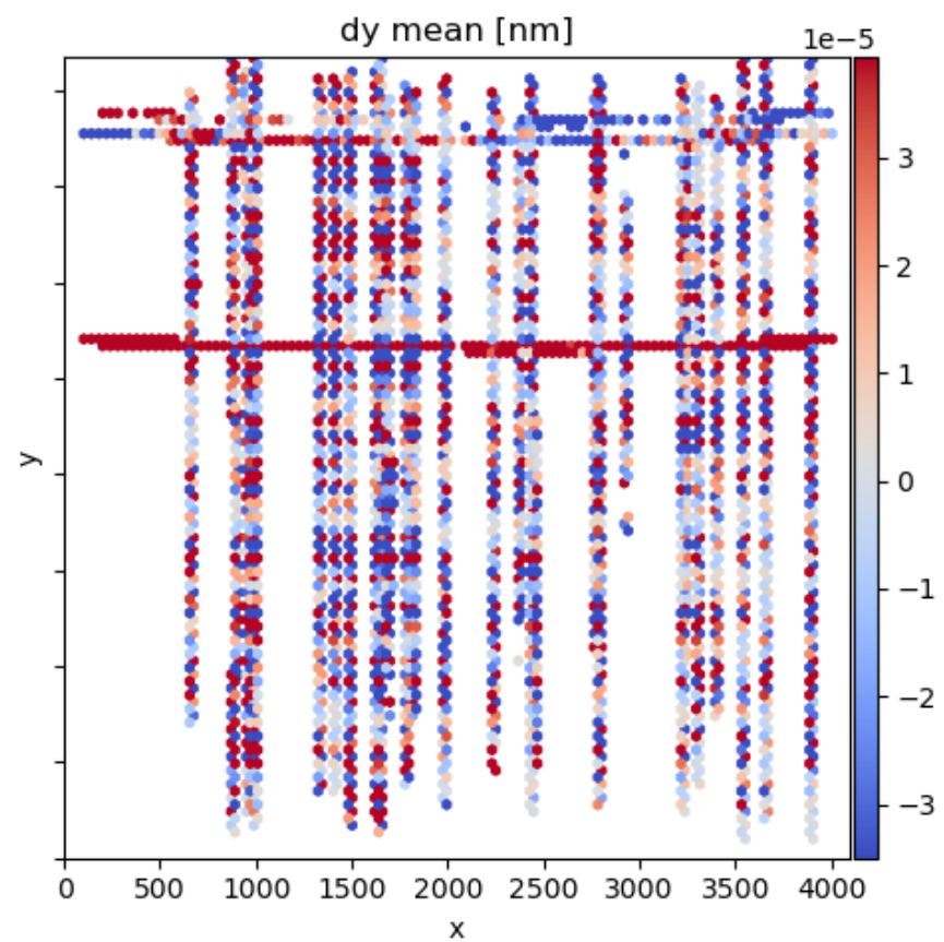
DETECTORMAP_USED residual (visit=97828, arm='b', spectrograph=1)
