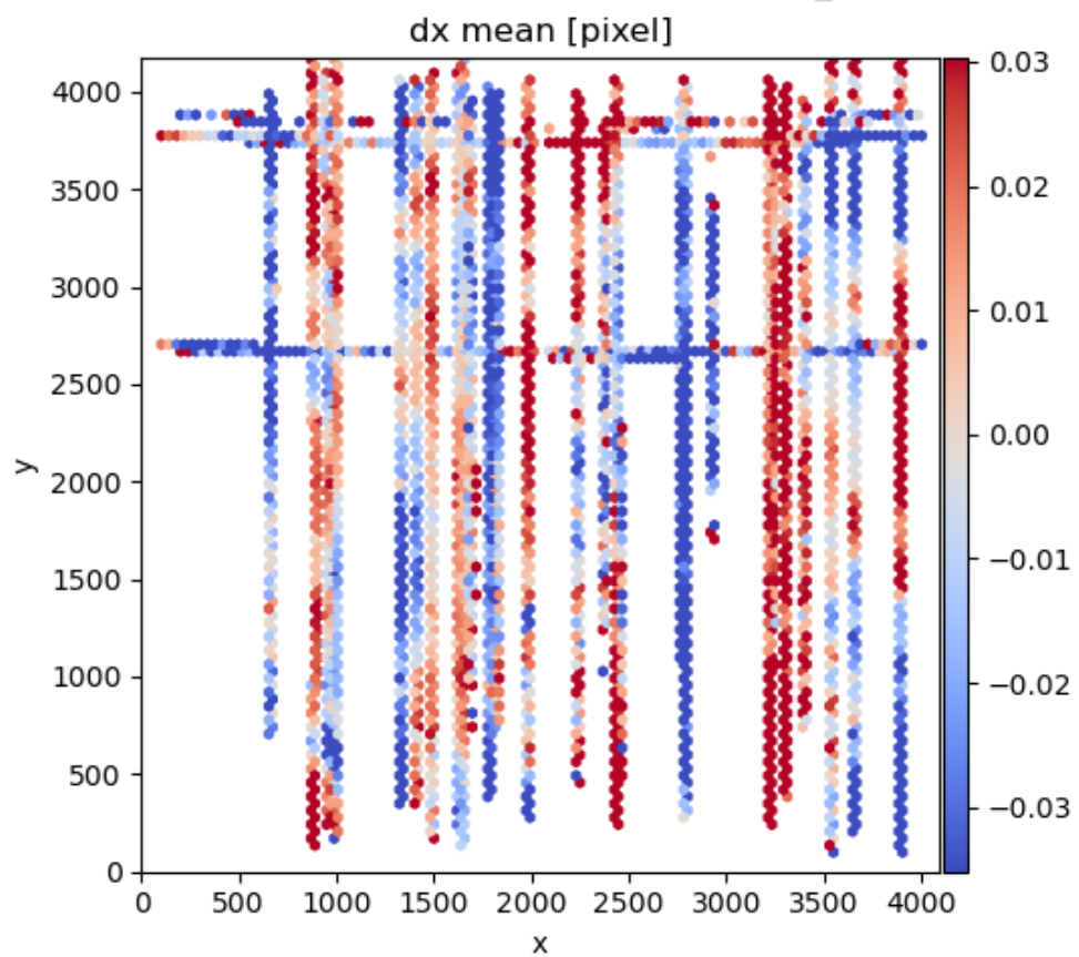
DETECTORMAP_USED residual (visit=97828, arm='b', spectrograph=1)
