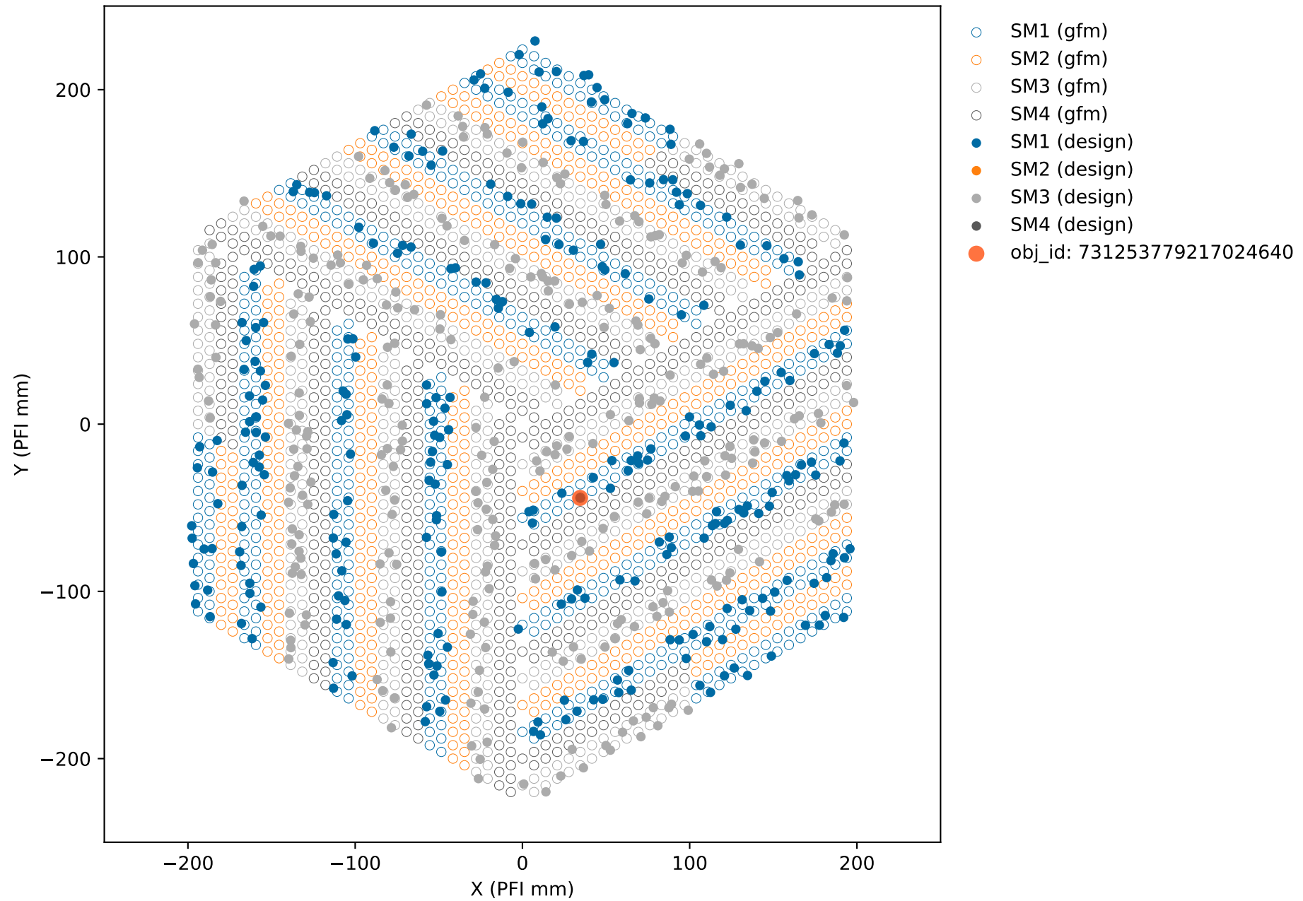
pfsDesign-0x413bcf208d3daa22.fits
