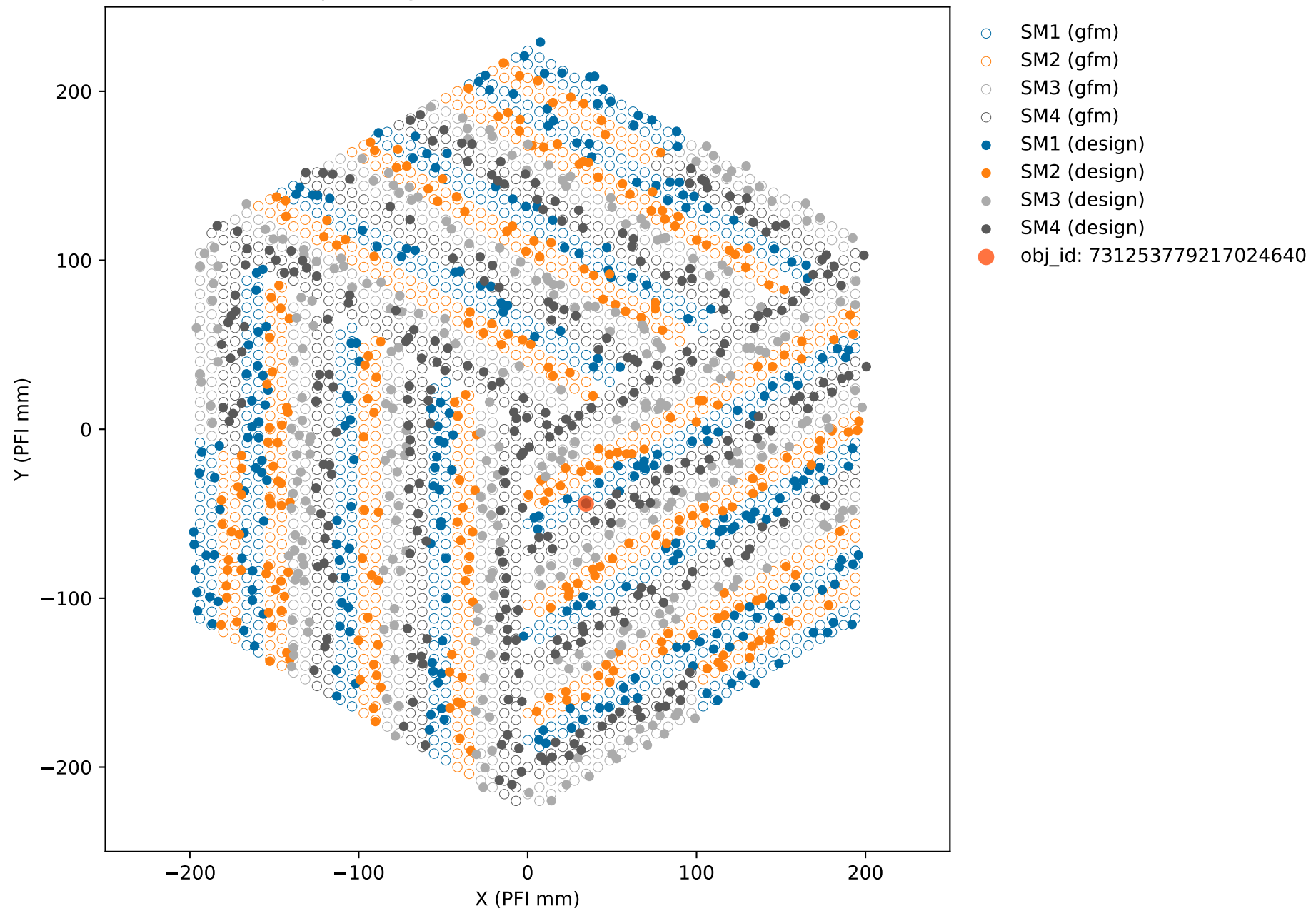
pfsDesign-0x78e3b3034e015cf0.fits
